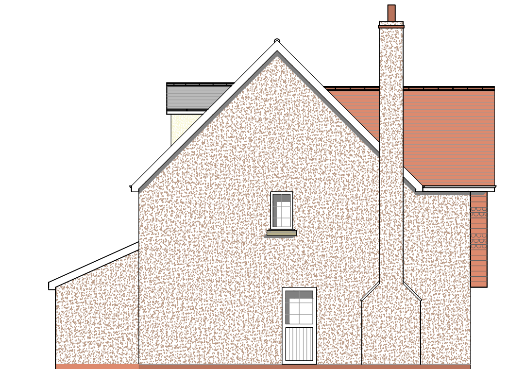
3 The Oakwood Side Elevation C 1:100
